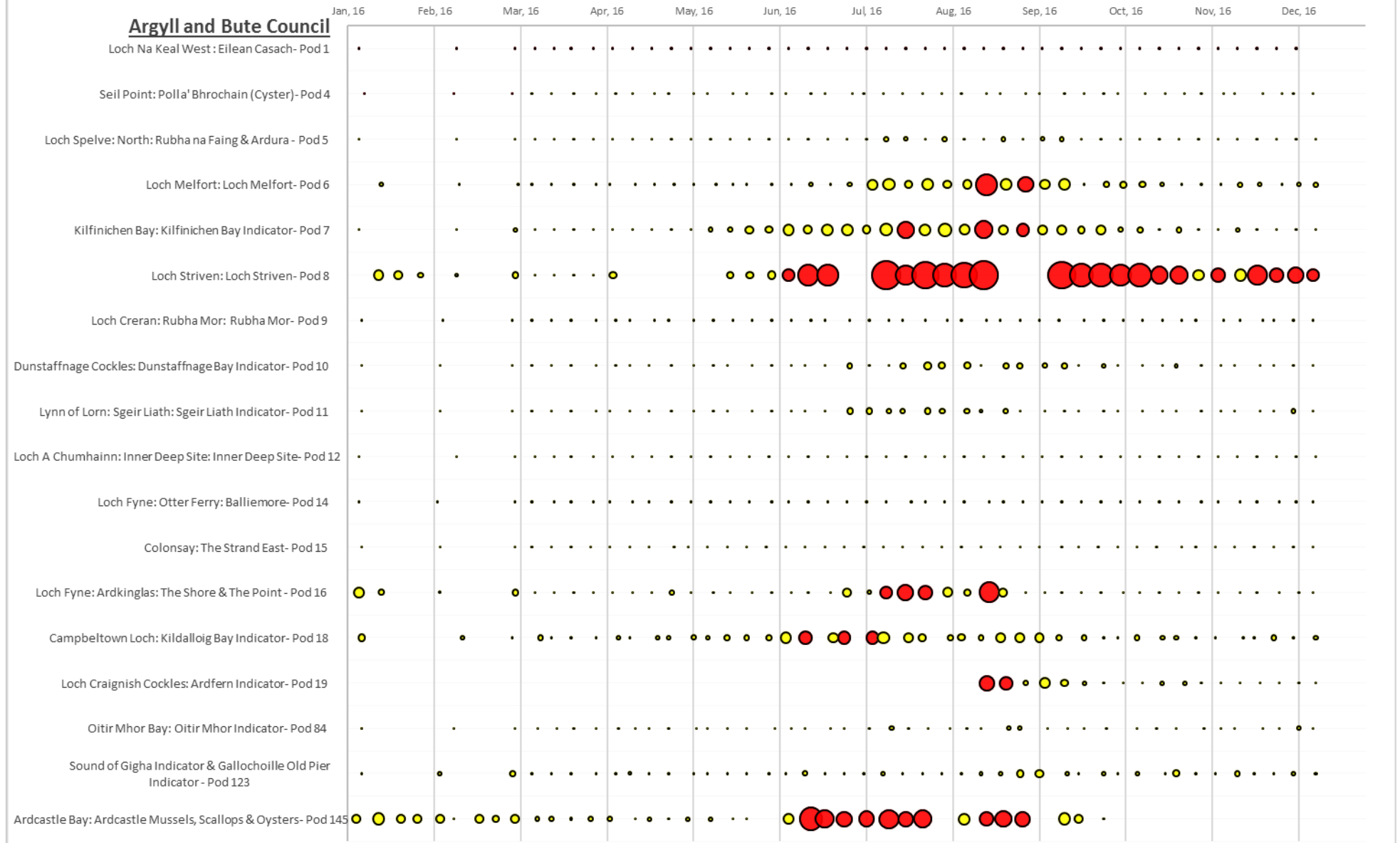
Figure 3: Concentrations of OA/DTX/PTX group toxins from January to December 2016
