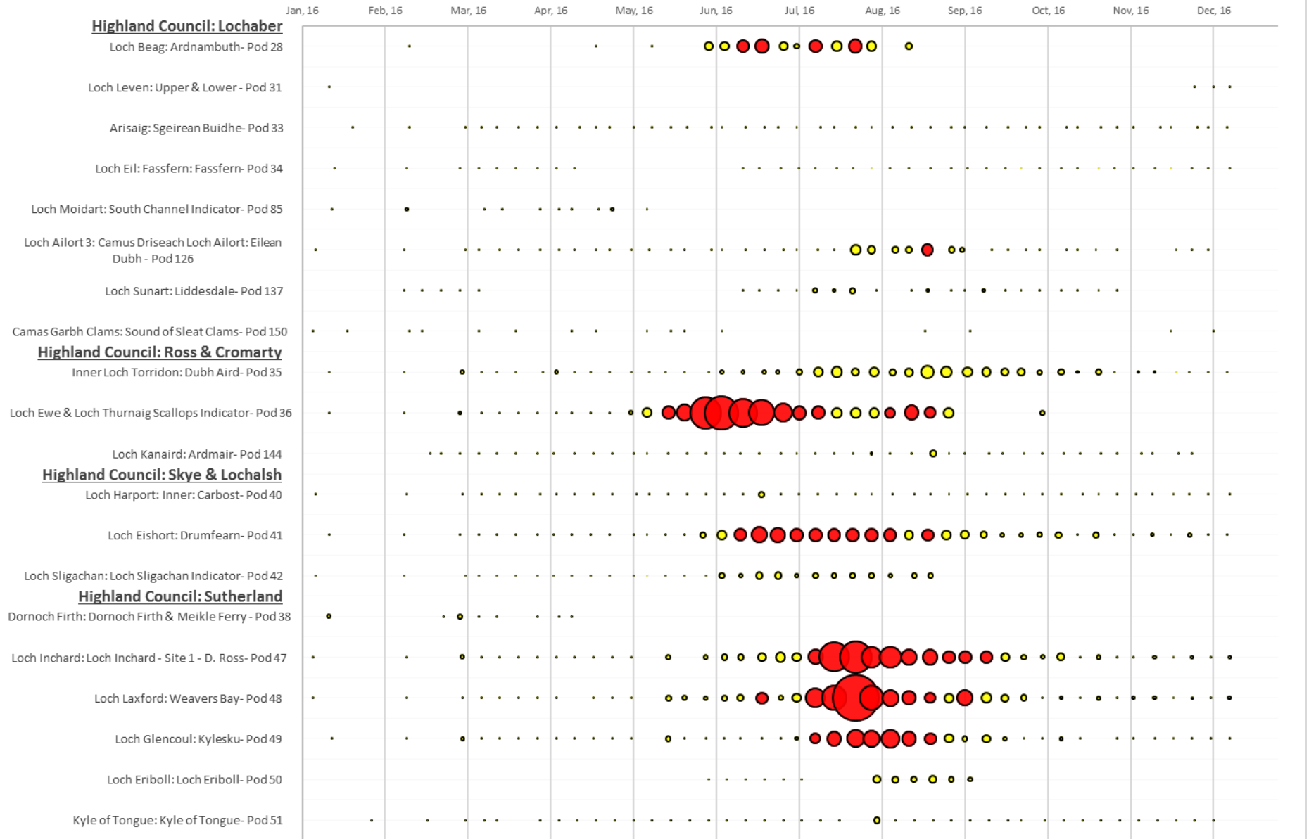
Figure 3: Concentrations of OA/DTX/PTX group toxins from January to December 2016 (continued)
