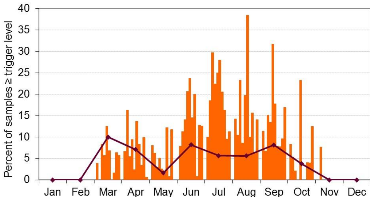
Figure 22: The percentage of samples in which Pseudo-nitzschia spp. equalled or exceeded the trigger level of 50,000 cells/L in 2016 is indicated by the line. For comparison, the bars show the percentage of samples in which Pseudo-nitzschia spp. equalled or exceeded the trigger level between 2006 and 2015.
