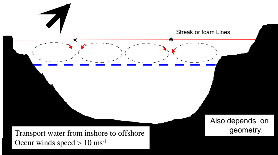
Figure 2: Schematic of wind driven 'wind row' currents. View is down the loch. The dotted blue line indicates the depth of the surface fresh(er) water layer usually found in sea lochs.
