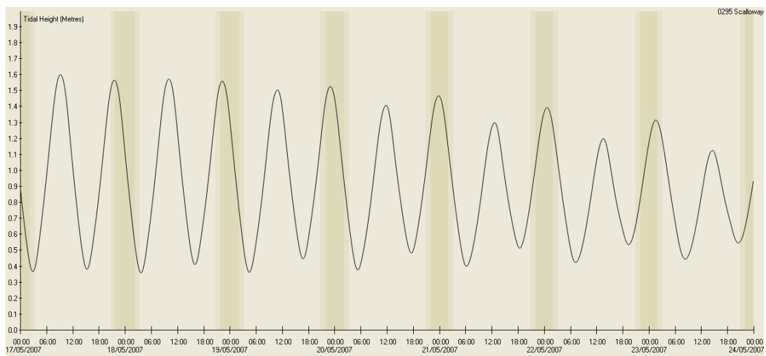
Figure 13.3 Scalloway tidal curves
