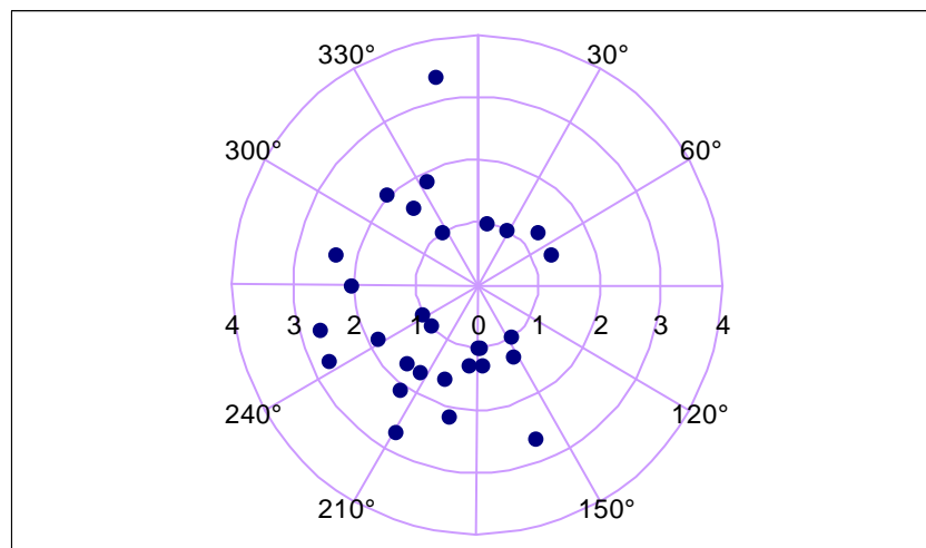
Figure 11.28 Polar plot of log 10 E. coli result by wind direction (Galtaskerry)
