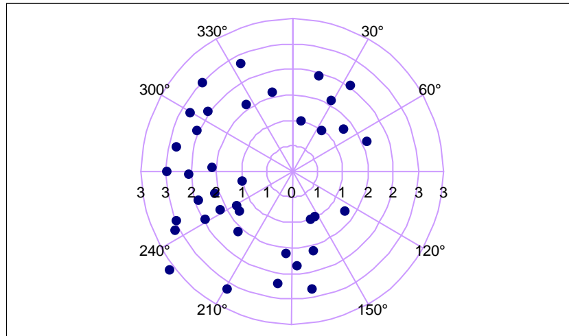
Figure 11.27 Polar plot of log 10 E. coli result by wind direction (Linga)
