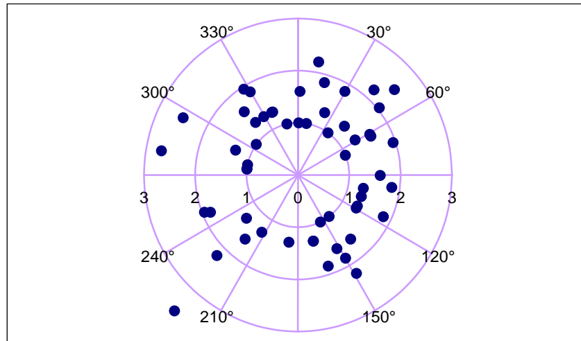
Figure 11.26 Polar plot of log 10 E. coli result by tidal state (Riskaness)
