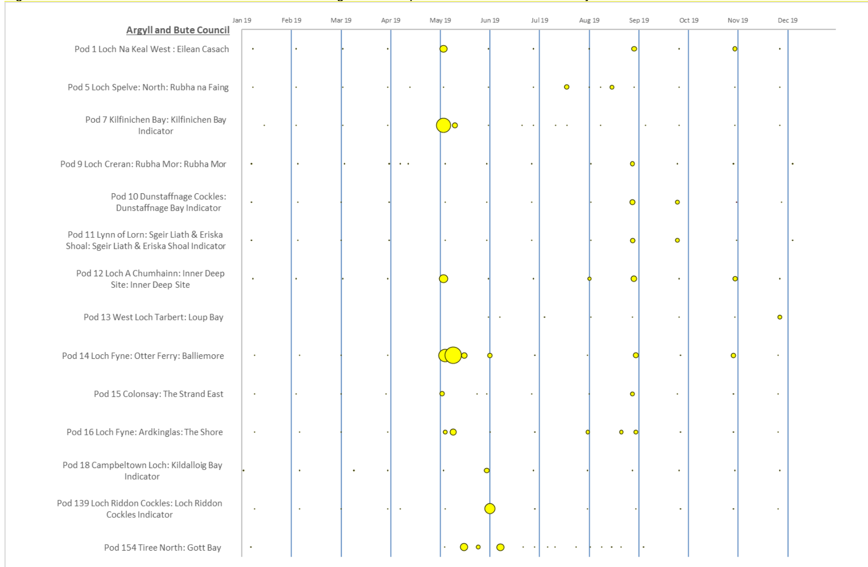
Figure 20. Concentrations of ASP toxins in sites recording results at quantifiable levels from January to December 2019
