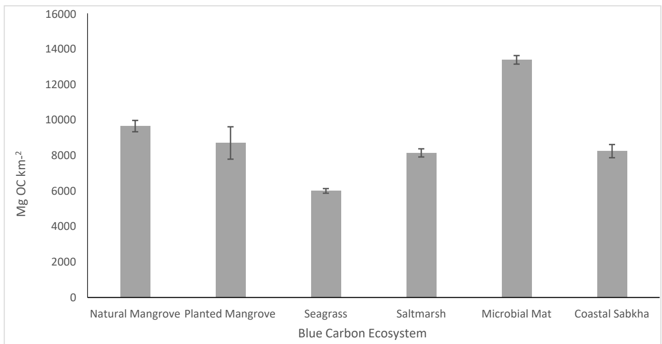
Figure 4: Soil Organic Carbon stocks (up to 1 m depth) in Mg C/km 2 for each blue carbon ecosystem. Error bars = standard error.
