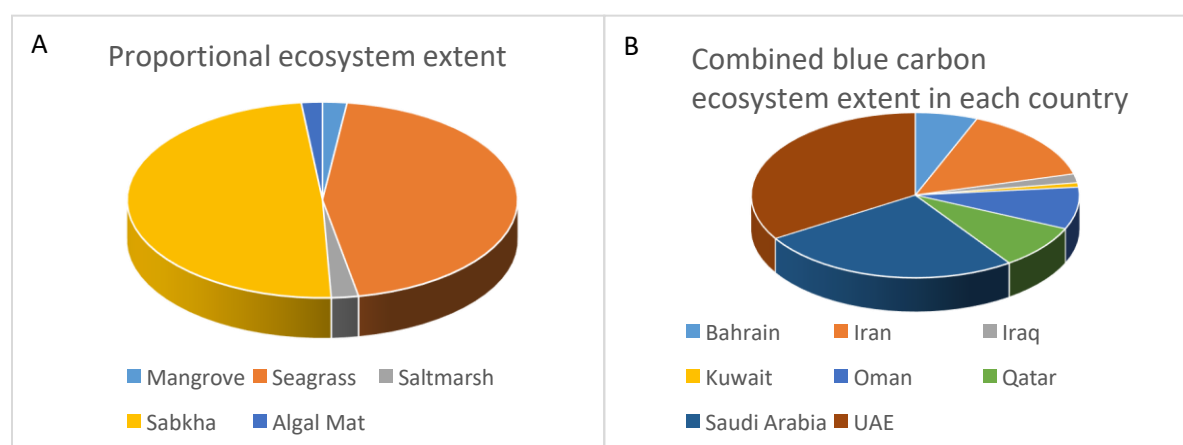
Figure 3: Proportion of total blue carbon habitat area covered by each type (A) and comparison between countries (B).
