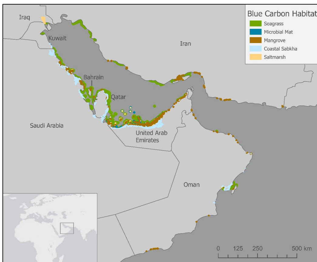
Figure 2: Distribution of blue carbon ecosystems of the ROPME Sea Area as summarised by the ROPME Technical Support Group for Blue Carbon in January 2020. The lack of information in some areas (i.e., saltmarsh or coastal sabkhas on the coast of Iran) may not indicate the absence of such ecosystem, rather the lack of spatial information for those ecosystems.
