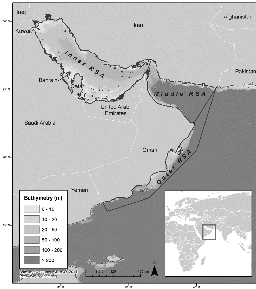
Figure 1: The coverage of the ROPME Sea Area (RSA) including geographical divisions. The RSA is bounded in the south by the rhumb lines 16° 39'N, 53° 3'30"E; 16° 00'N, 53°25'E; 17°00'N, 56° 30'E; 20° 30'N; 60° 00'E; 25° 04'N; 61° 25'E, comprising three geographically and environmentally distinct parts: the Inner RSA (I-RSA), the Middle RSA (M-RSA) and the Outer RSA (O-RSA).
